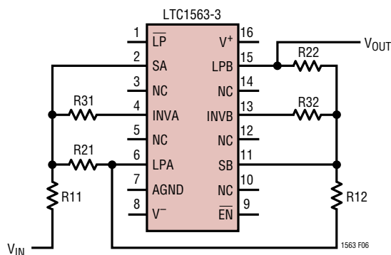
Figure 6. 4th Order Filter Connections (Power Supply, Ground, \overline{\text{EN}} and \overline{\text{LP}} Connections Not Shown for Clarity). Table 2 Shows Resistor Values
