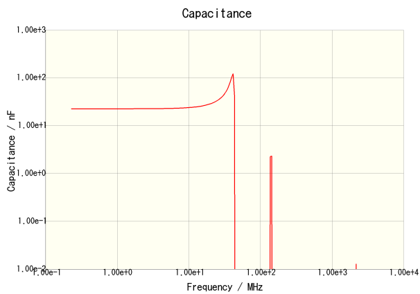
C2012C0G1E223J125AA
