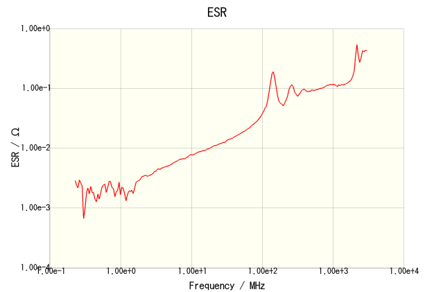
C2012C0G1E223J125AA
