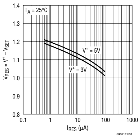
Figure 1. V^+ - V_{\text{SET}} Variation with I_{\text{RES}}
