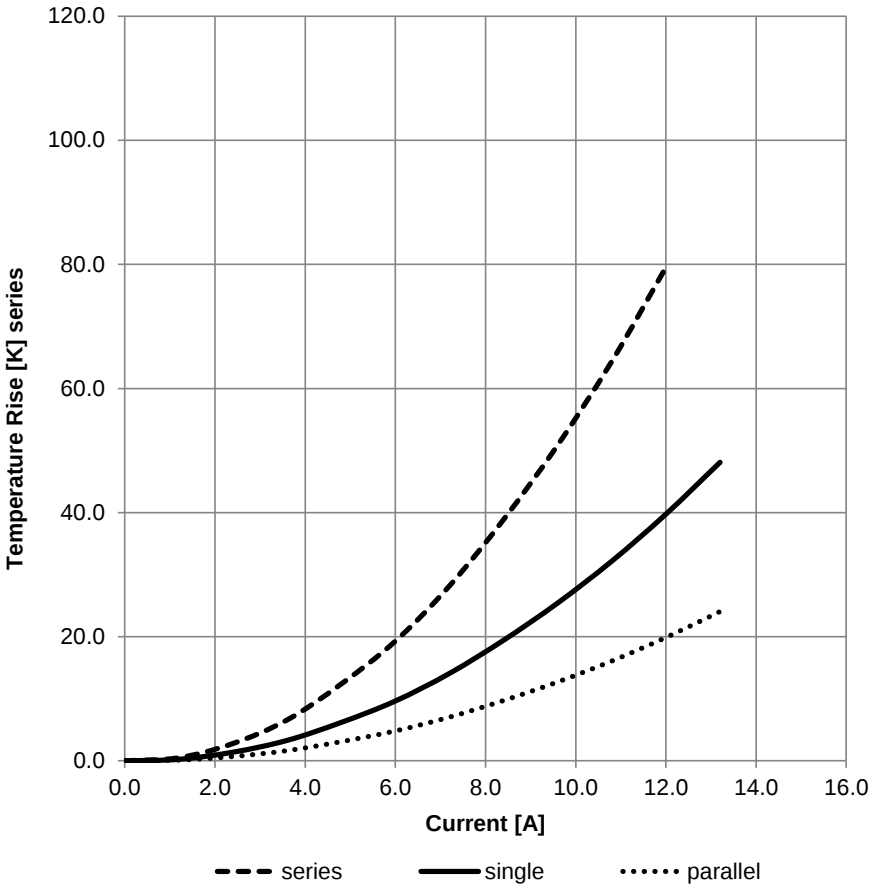
Typical Temperature Rise vs. Current Characteristics:
