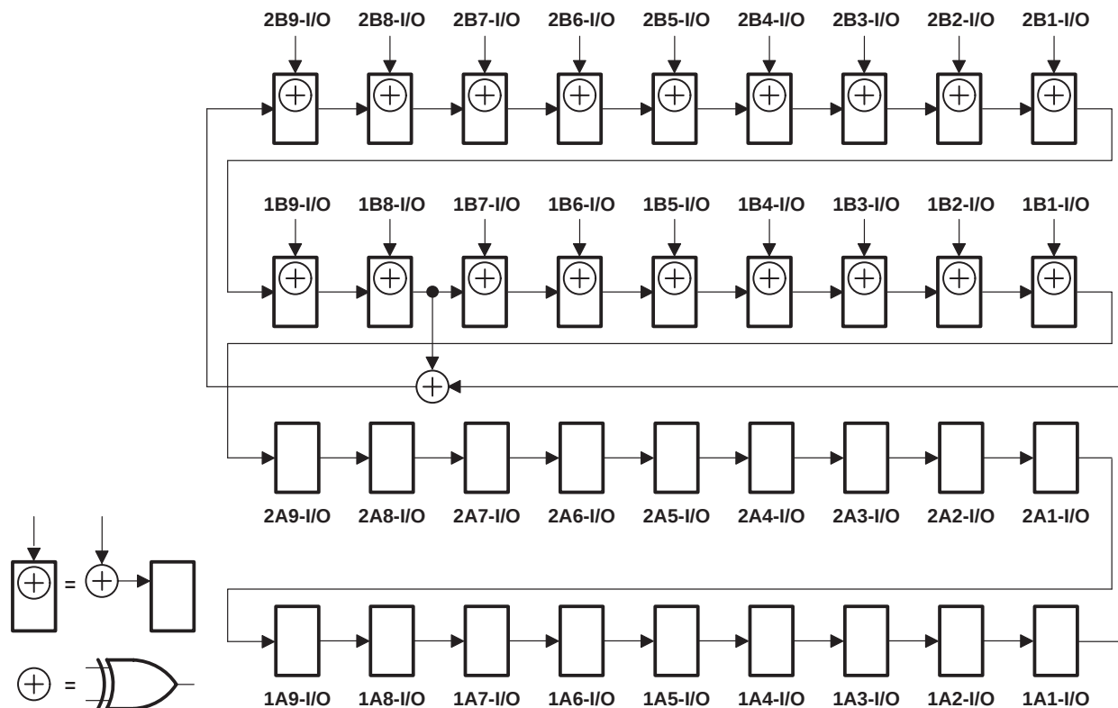
Figure 8. 36-Bit PSA Configuration ( \overline{1OEAB} = \overline{2OEAB} = 1 , \overline{1OEBA} = \overline{2OEBA} = 0 )
