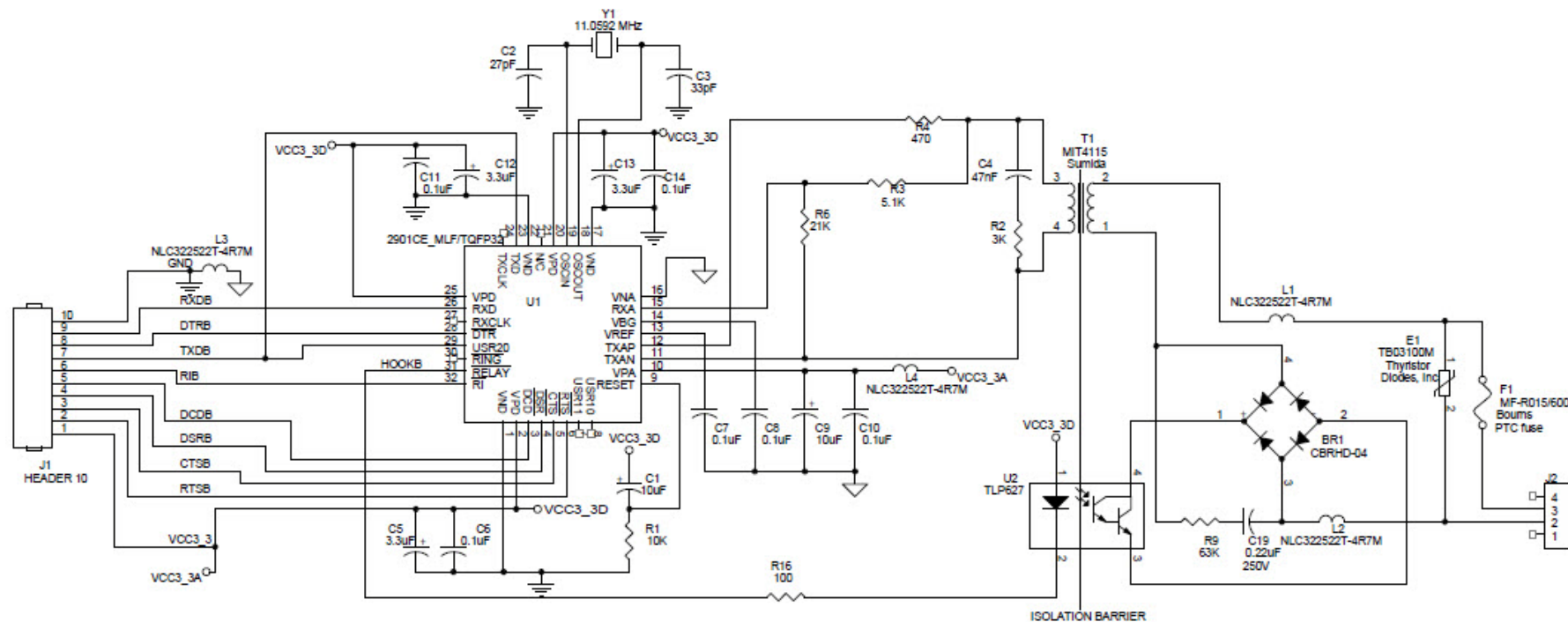
Figure 3: Low Cost Design Using DSP Ring and Status Monitoring
