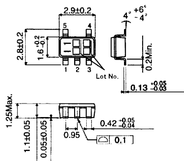
BU4S11G2(SSOP5)(UNIT:[mm])
