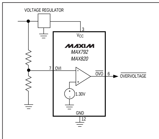
Figure 6. Detecting an Overvoltage Condition
