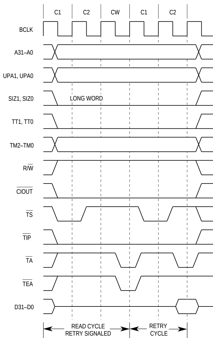
Figure 7-28. Retry Read Transfer Timing
