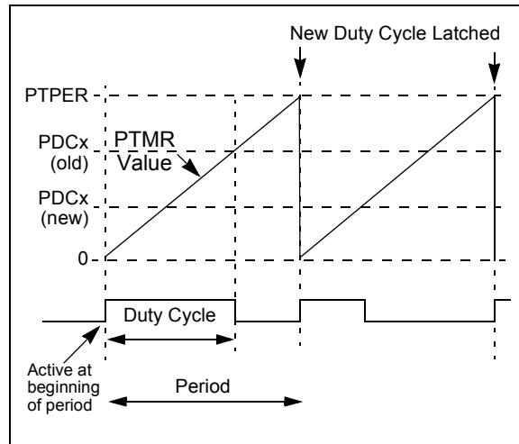
FIGURE 17-12: EDGE-ALIGNED PWM
