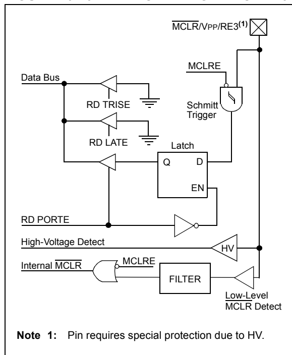
FIGURE 10-29: BLOCK DIAGRAM OF RE3
