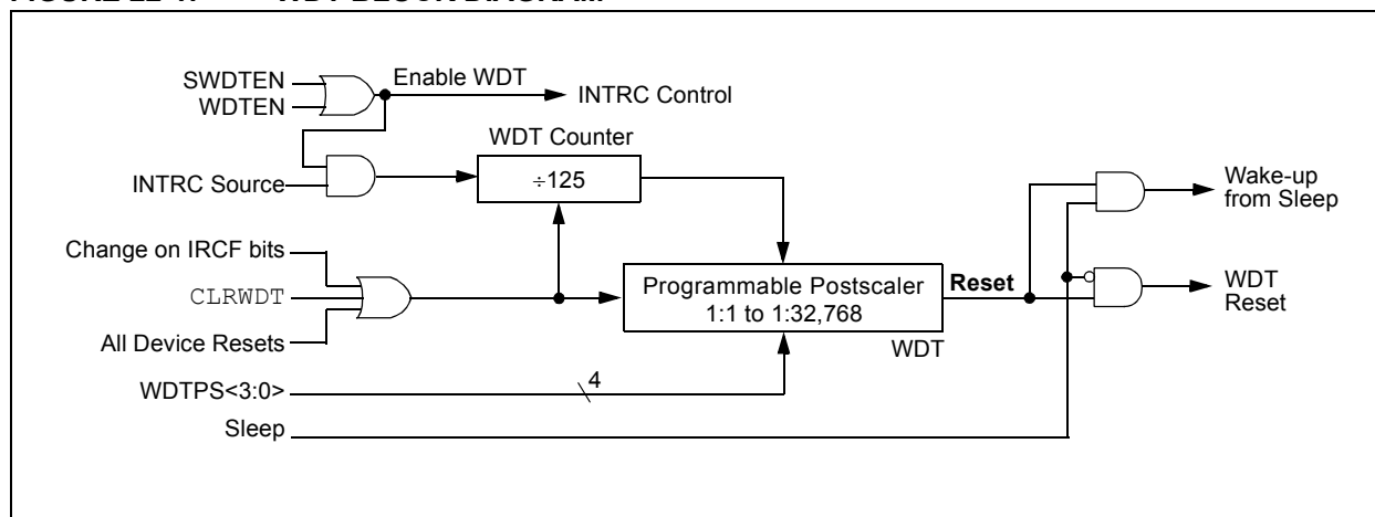
FIGURE 22-1: WDT BLOCK DIAGRAM
