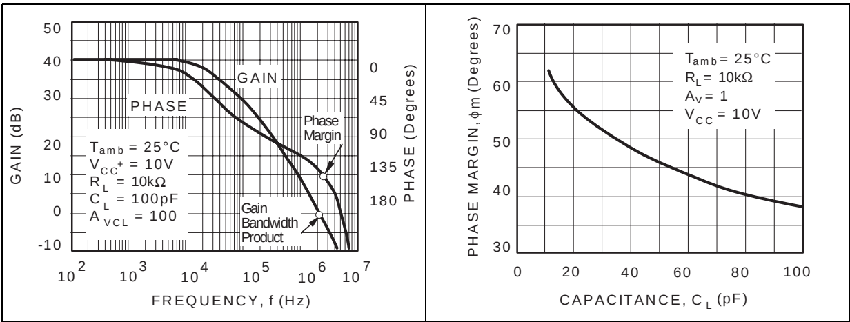
Figure 9. Open loop frequency response and phase shift
