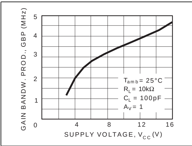
Figure 11. Gain bandwidth product vs. supply voltage
