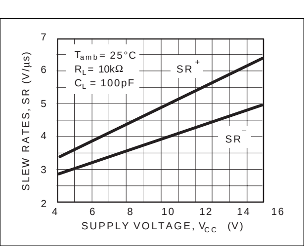
Figure 12. Slew rate vs. supply voltage
