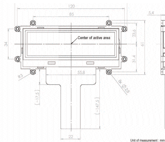
Reflective Version (P/N BT21015)
