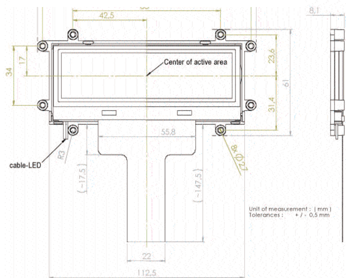
LED Version (P/N BT21016)
