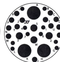
25-20 - 25-20*• No. of Contacts 3 #8 Twinax, 13 #16, 4 #12 Coax, 10 #20 Service Ratings N / Coax / Twinax
