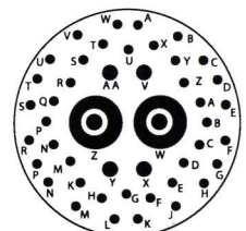
25-46 - 25-46 No. of Contacts 40 #20, 4 #16, 2 #8 Service Ratings Twinax
