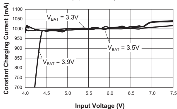
Constant Charging Current vs. Input Voltage ( R_{SET} = 1.58K\Omega )
