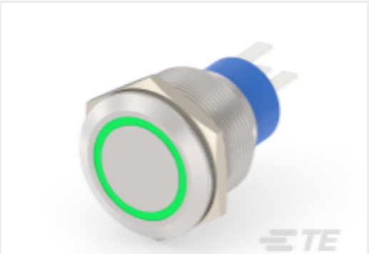
TE Part #1-2213772-5 AV22 SPM 3A MOVE RING LED GREEN 24V
