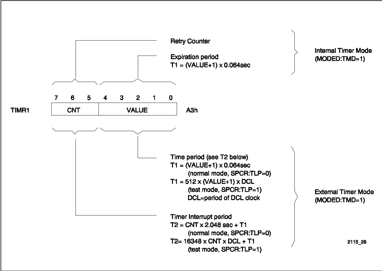
Figure 48 Timer 1 Register
