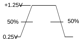
Figure 26. HSTL I/II I/O Input Waveform
