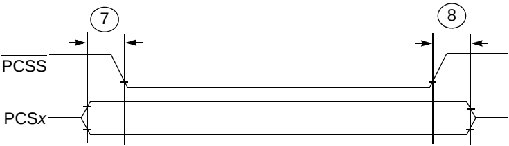
Figure 32. DSPI PCS Strobe (PCSS) Timing
