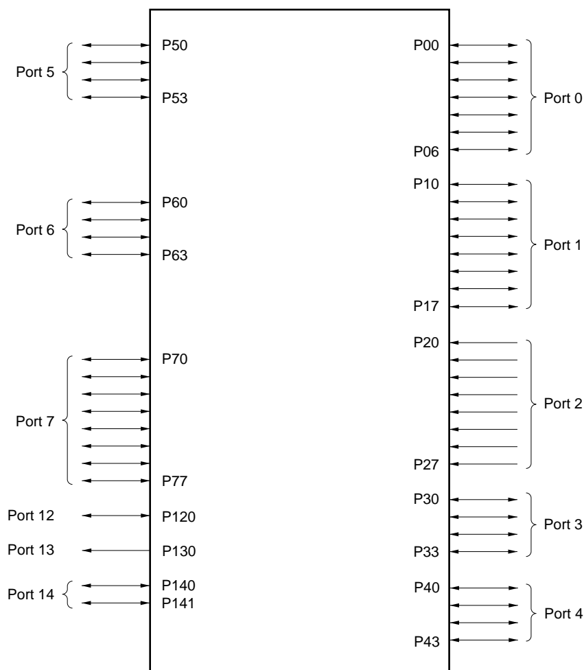
Figure 4-1. Port Types
