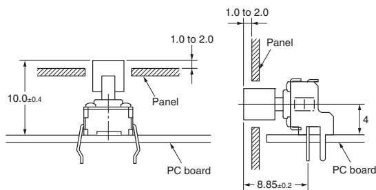
Reference Dimensions
