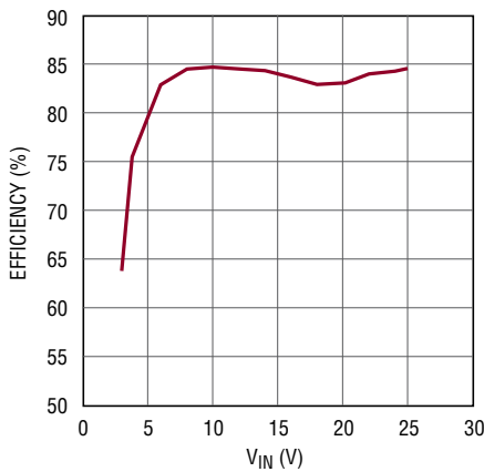
Efficiency vs V_{IN} , Buck-Boost Mode, 9.7V at 350mA LED String
