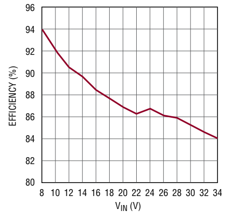
Efficiency vs V_{IN} , Buck Mode, 6.7V at 350mA LED String
