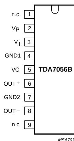
Fig.2 Pin configuration.
