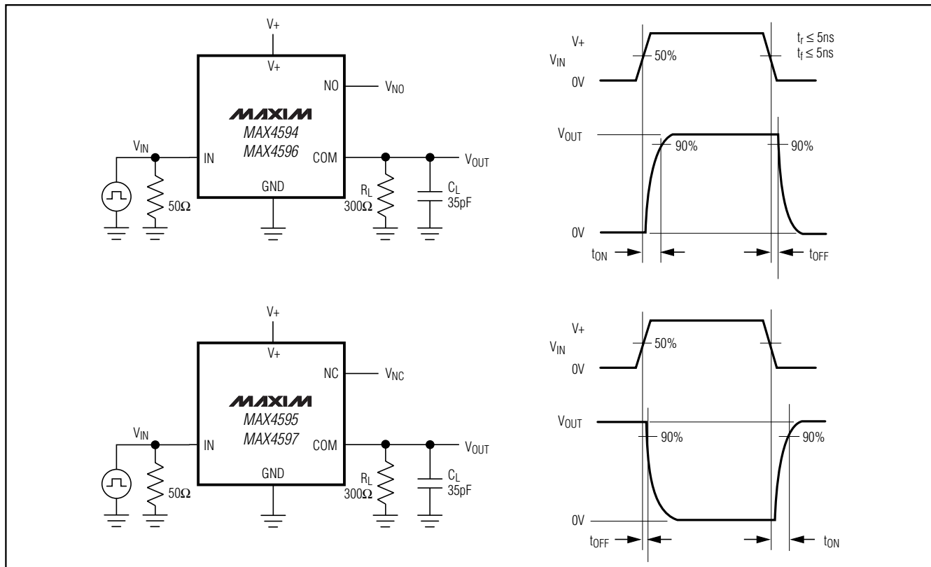
Figure 3. Switching Times
