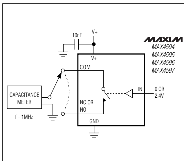
Figure 5. Channel On-/Off-Capacitance
