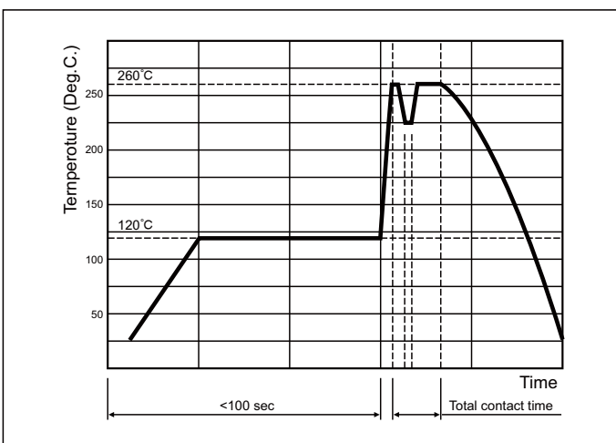
Figure. Wave soldering
