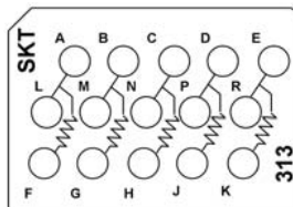
CTJ420E313 Five 100 kΩ Resistors, 1/4 W
