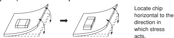
[Chip Mounting Close to Board Separation Point]
