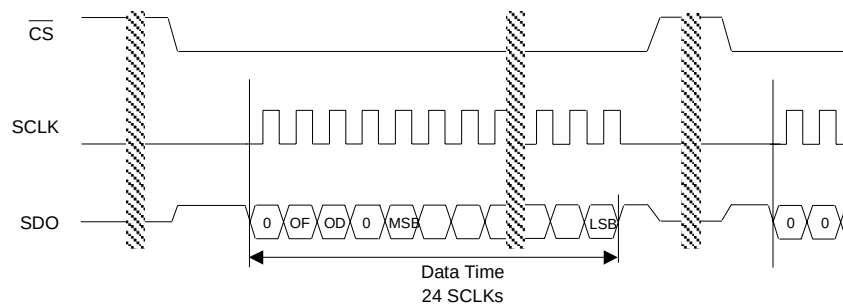
Figure 19. Data Word Timing for the CS5513.
