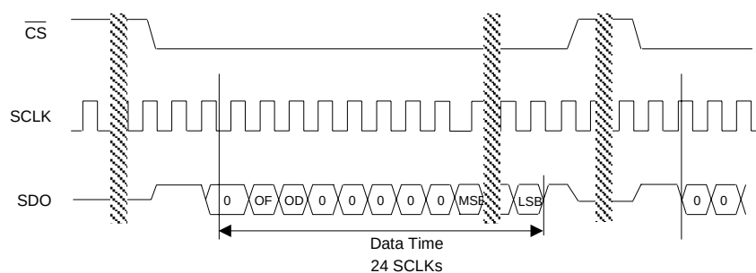
Figure 16. Data Word Timing for the CS5510.
