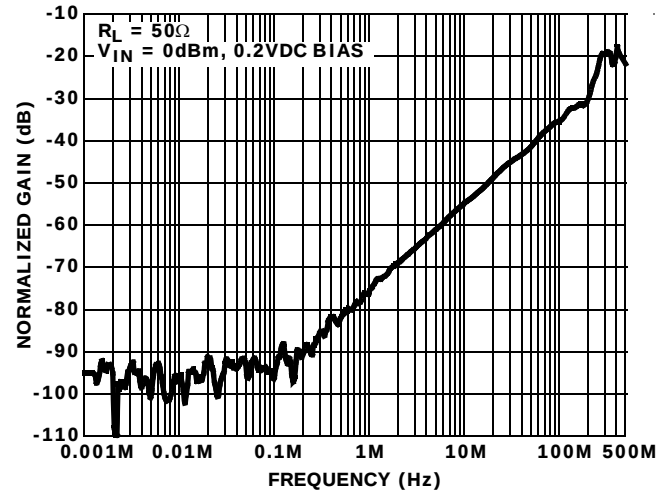
FIGURE 17. OFF-ISOLATION
