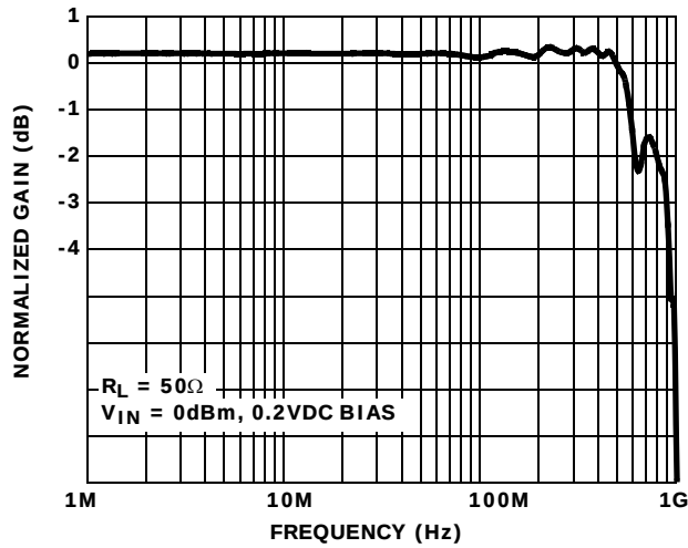
FIGURE 16. FREQUENCY RESPONSE
