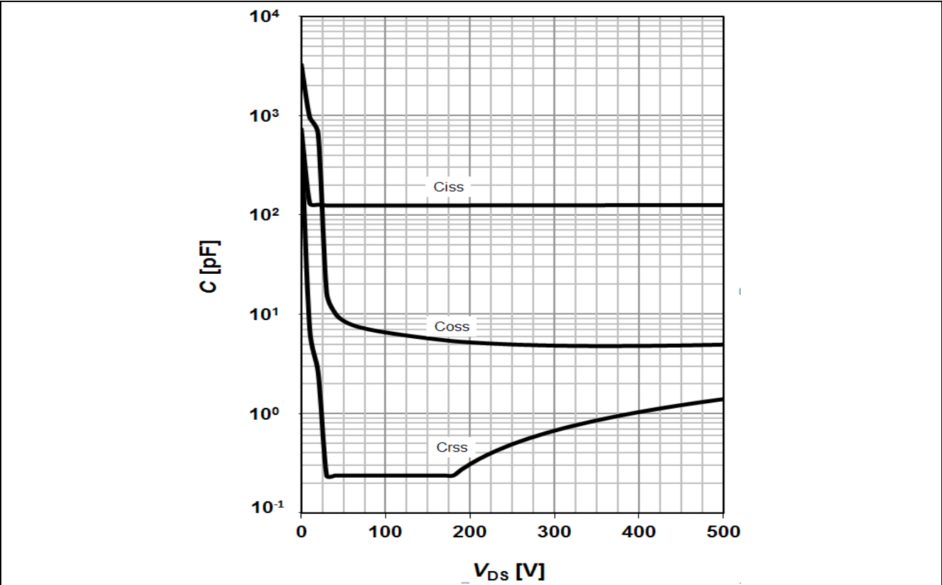
Figure 37 Typical CoolMOS™ capacitances of ICE5QR2280AZ ( C=f(V_{DS}); V_{GS}=0 V; f=250 kHz)
