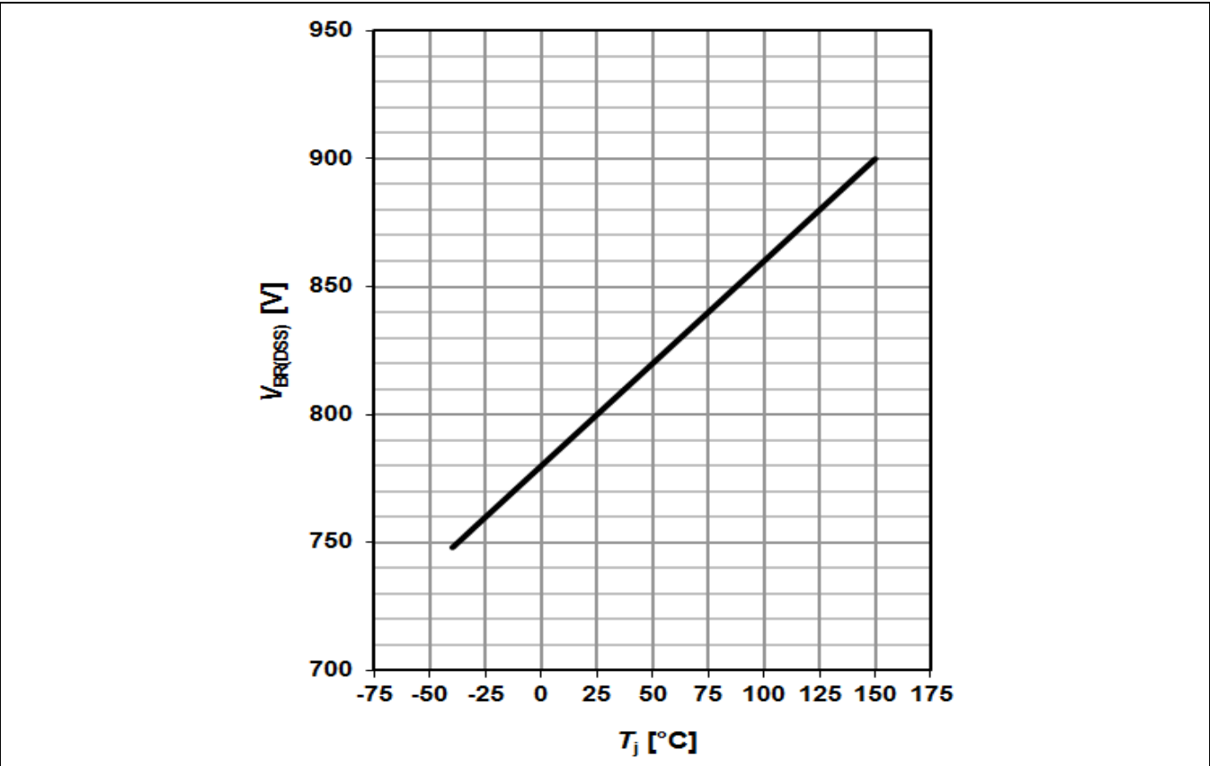
Figure 33 Drain-source breakdown voltage ICE5QRxx80Ax; V_{BR(DSS)}=f(T_J) , I_D=1 mA
