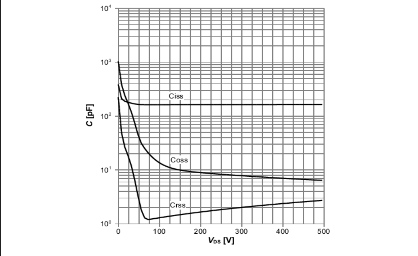
Figure 36 Typical CoolMOS™ capacitances of ICE5QR2270AZ ( C=f(V_{DS}); V_{GS}=0 V; f=1 MHz)
