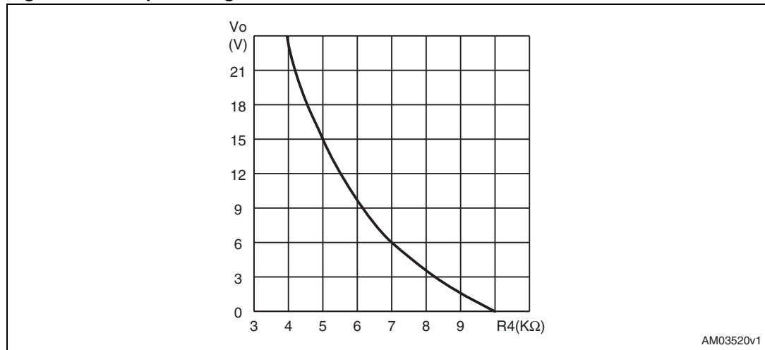
Figure 38. Output voltage vs. R4
