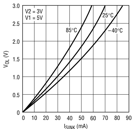
RST, WDO, COMPM Voltage Output Low vs Output Sink Current
