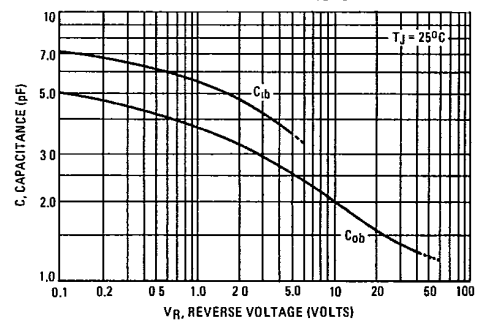
FIGURE 6 - CAPACITANCES
