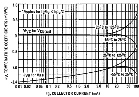
FIGURE 4 - TEMPERATURE COEFFICIENTS
