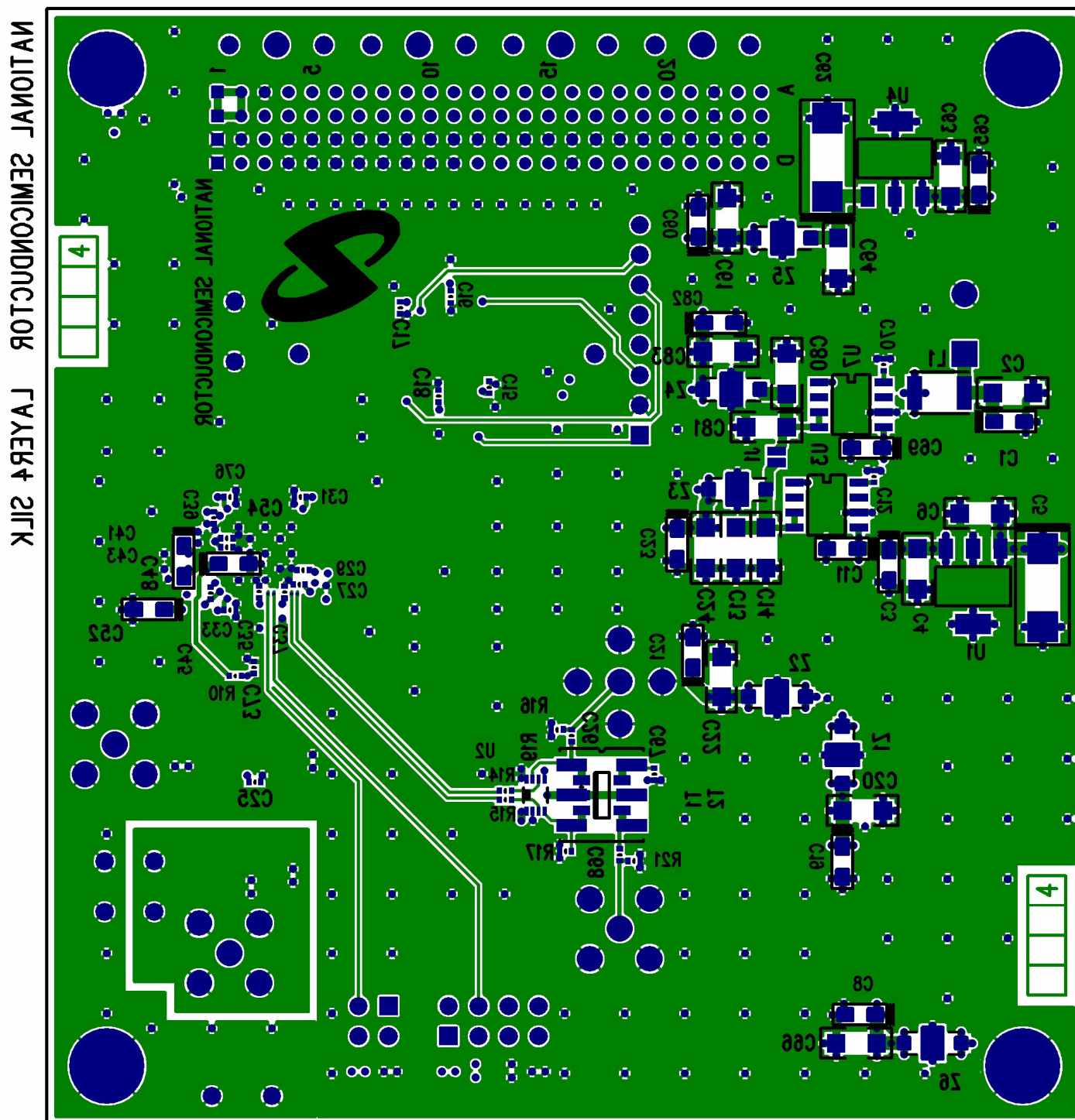
Figure 9. Layer 4 - Signal
