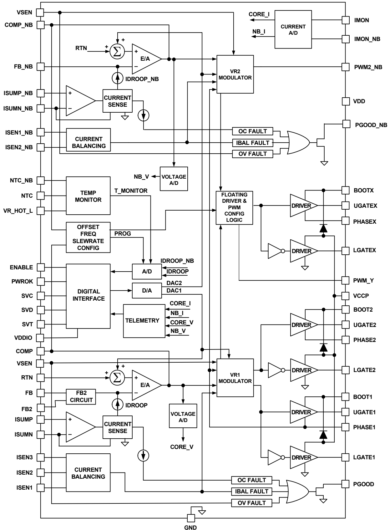
FIGURE 7. BLOCK DIAGRAM
