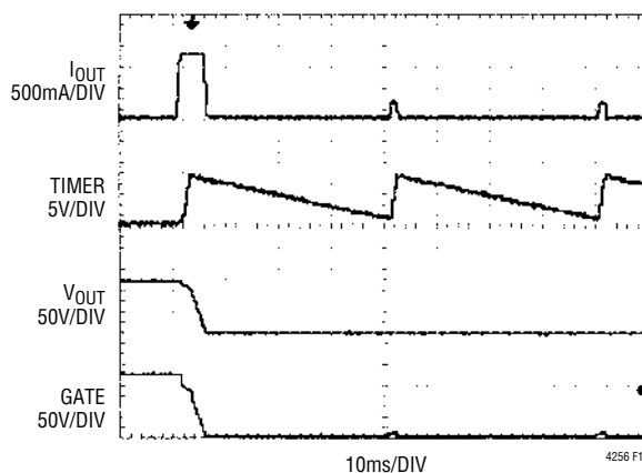
Figure 11. RETRY Waveforms
