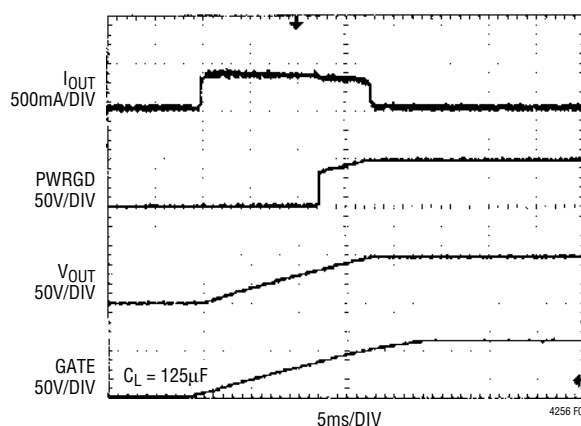
Figure 6. Start-Up Waveforms
