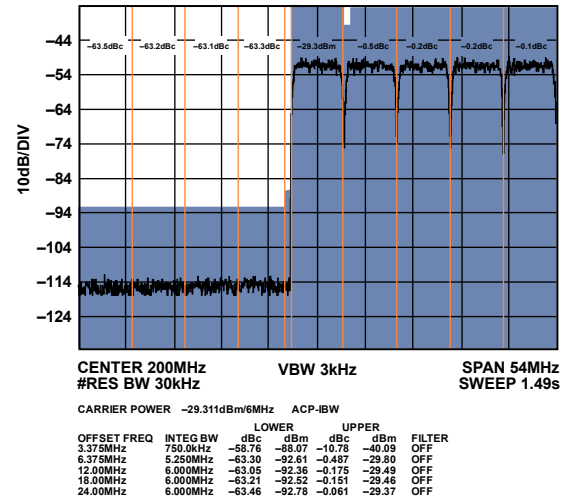
Figure 61. Low Band Narrow-Band ACLR (Worst Side)
