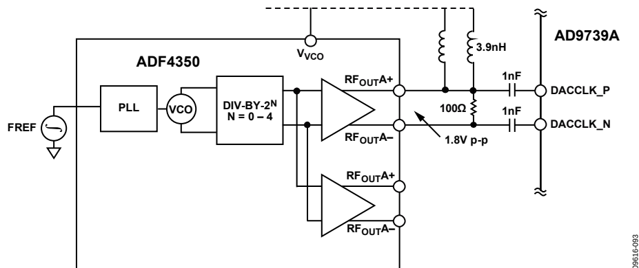
Figure 90. ADF4350 Interface to the AD9739A CLK Input
