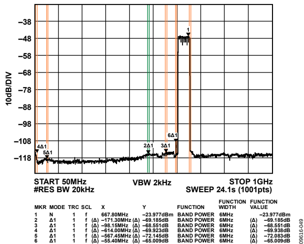
Figure 47. Mid Band Wideband ACLR
