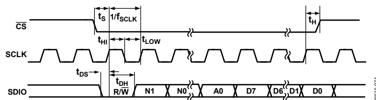
Figure 71. SPI Write Operation Timing
