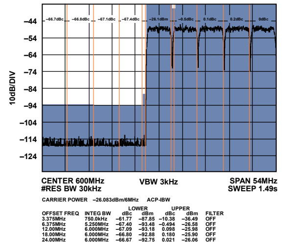
Figure 56. Mid Band Narrow-Band ACLR (Worst Side)
