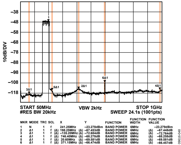
Figure 46. Low Band Wideband ACLR
