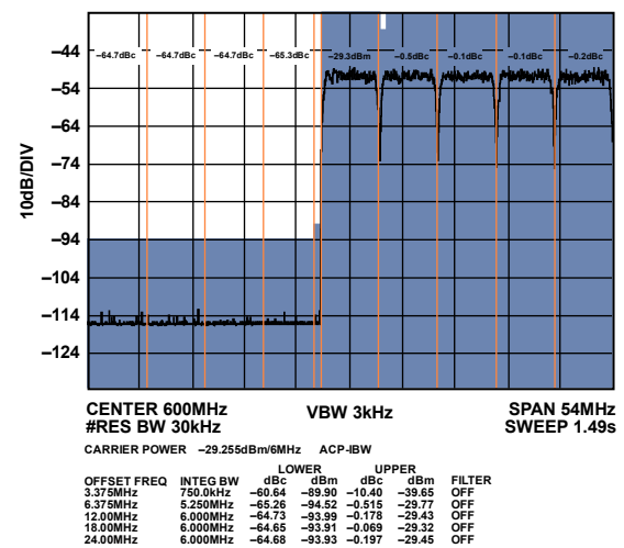
Figure 62. Mid Band Narrow-Band ACLR (Worst Side)
