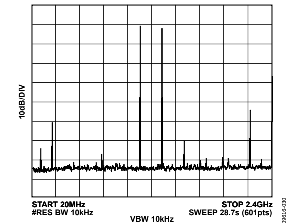
Figure 28. Single-Tone Spectrum in Mix Mode at f_{OUT} = 1.31 GHz, f_{DAC} = 2.4 GSPS
