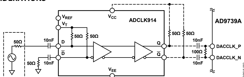
Figure 89. ADCLK914 Interface to the AD9739A CLK Input
