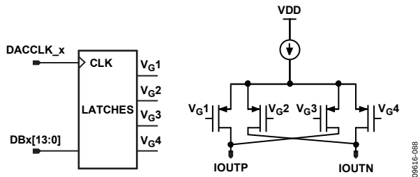
Figure 85. AD9739A Quad-Switch Architecture
