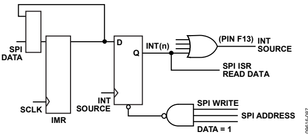
Figure 84. Interrupt Request Circuitry
