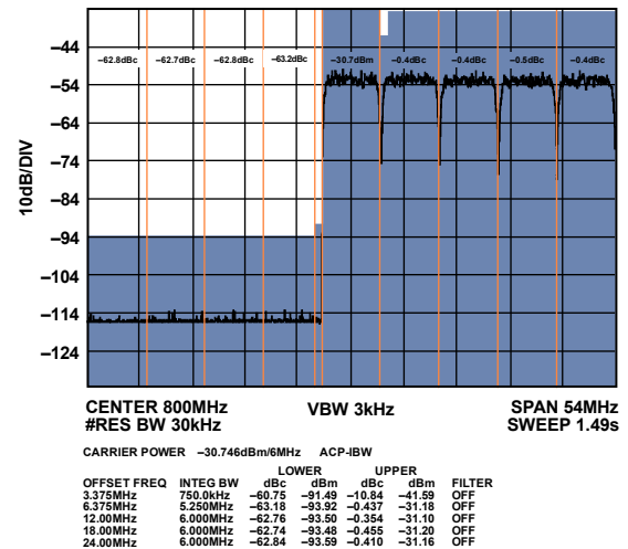
Figure 63. High Band Narrow-Band ACLR (Worst Side)
