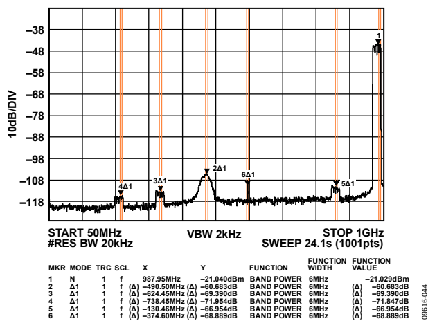
Figure 42. High Band Wideband ACLR
