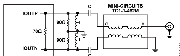
Figure 100. Recommended Mix-Mode Configuration Offering Extended RF Bandwidth Using a TC1-1-43A+ Balun
