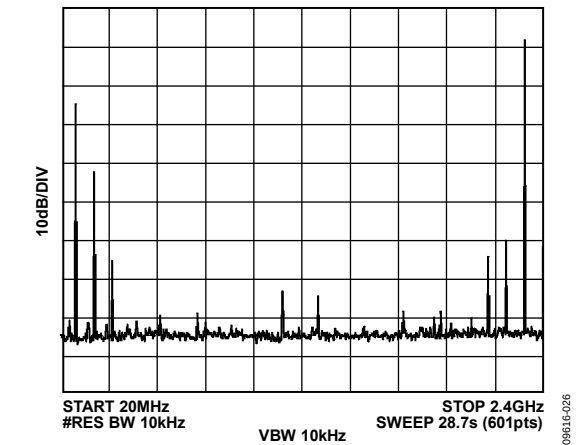
Figure 25. Single-Tone Spectrum at f_{OUT} = 2.31 GHz, f_{DAC} = 2.4 GSPS
