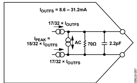
Figure 94. Equivalent DAC Output Circuit
