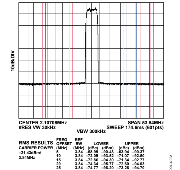
Figure 27. Typical Single-Carrier WCDMA ACLR Performance at 2.1 GHz, f_{DAC} = 2457.6 MSPS (Second Nyquist Zone)
