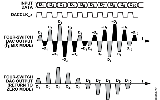
Figure 87. Mix-Mode and RZ DAC Waveforms
