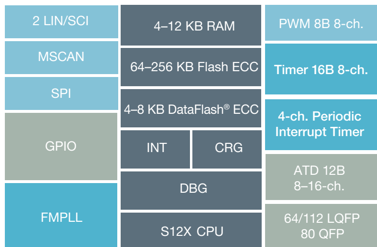
S12XS Family Block Diagram
