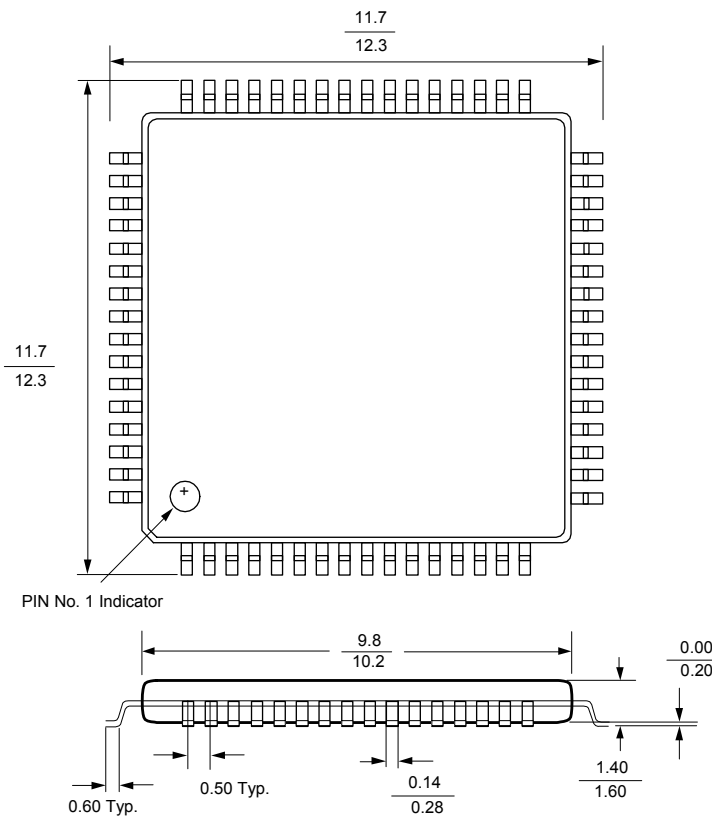
PACKAGE OUTLINE (LQFP 64)
