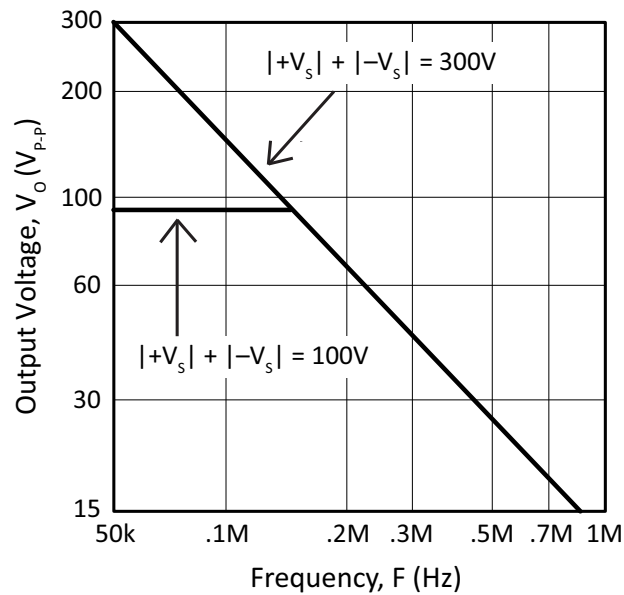
Figure 11: Slew Rate
