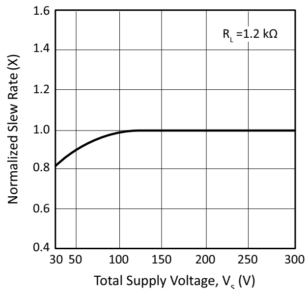
Figure 11: Slew Rate
