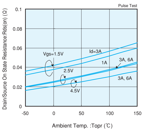
Drain/Source On-State Resistance vs. Ambient Temperature
