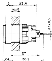
Terminals
