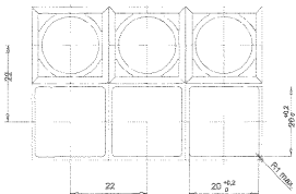
panel cutout
