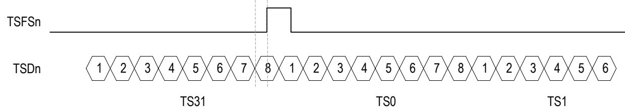
Figure 44. E1 Transmit Clock Master Mode - Functional Timing Example
