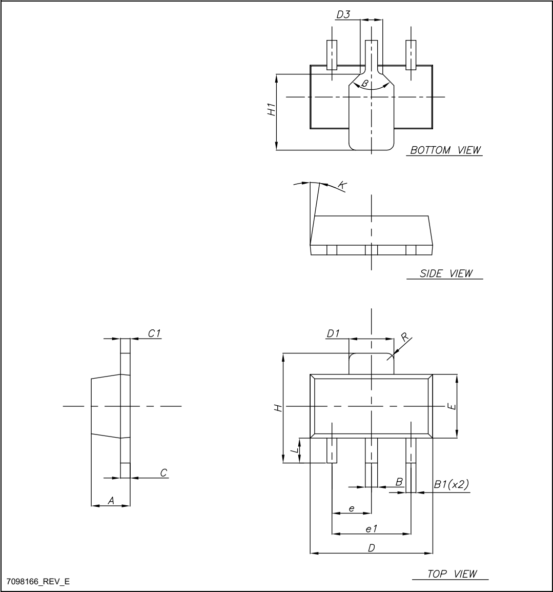
Figure 20. SOT-89 drawings
