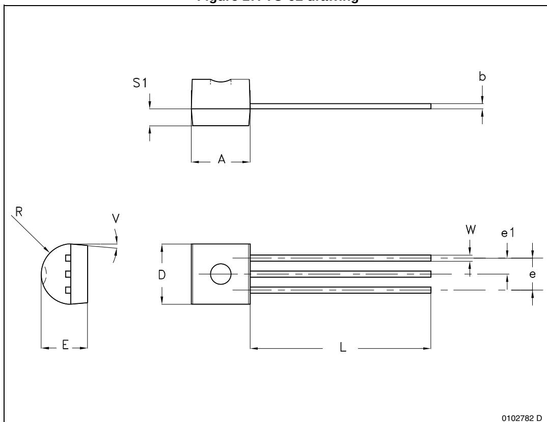
Figure 17. TO-92 drawing
