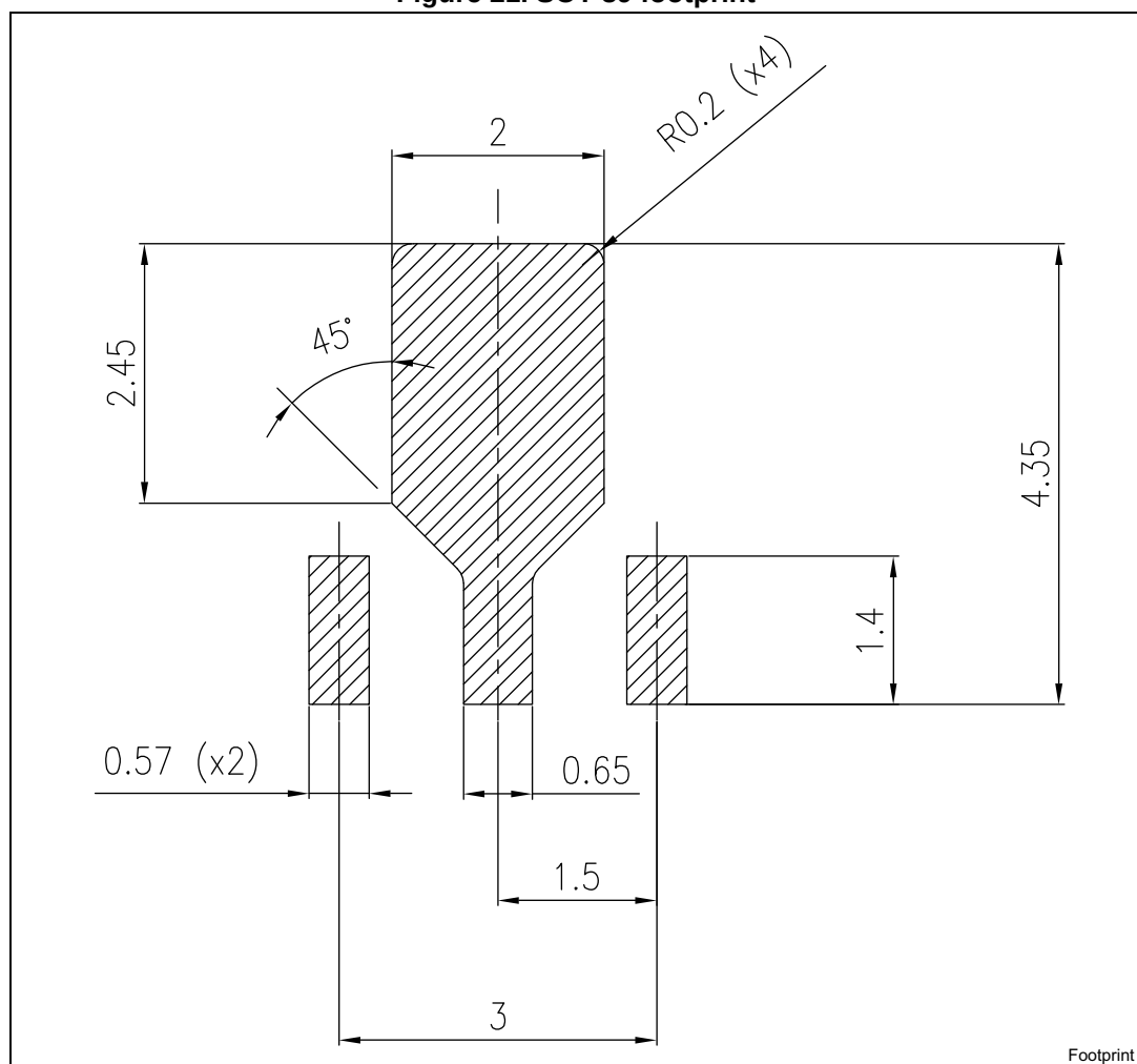
Figure 21. SOT-89 footprint
