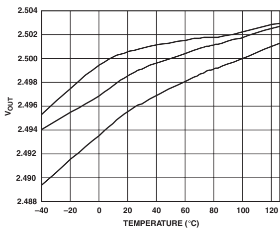
TPC 3. Typical Temperature Drift Characteristic Curves
