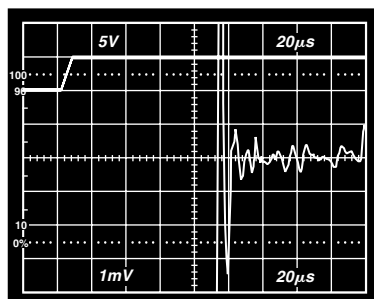
Figure 12c. Turn-On Settling
