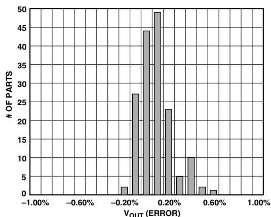
TPC 2. Typical Output Voltage Error Distribution
