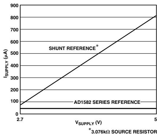
Figure 1. Supply Current ( \mu A) vs. Supply Voltage (V)
