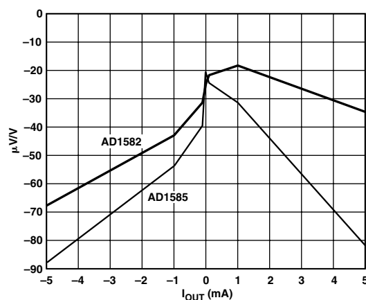
TPC 5. Line Regulation vs. I_{LOAD}
