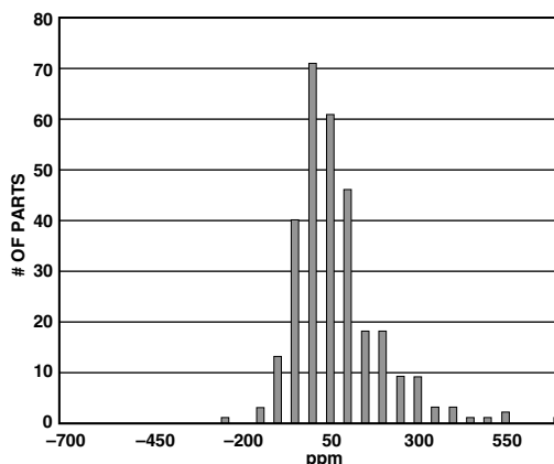
Figure 6. Output Voltage Hysteresis Distribution
