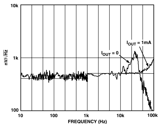
TPC 6. Noise Spectral Density
