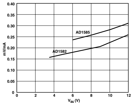
TPC 4. Load Regulation vs. V_{IN}
