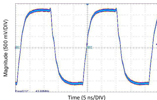
Figure 5-19. DS90UR124 PCLK Output at 43MHz
