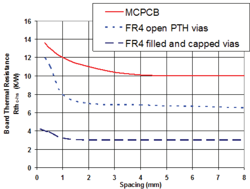
Figure 24. Comparison R_{\theta_{c-hs}} of various board technologies as a function of LED spacing.
