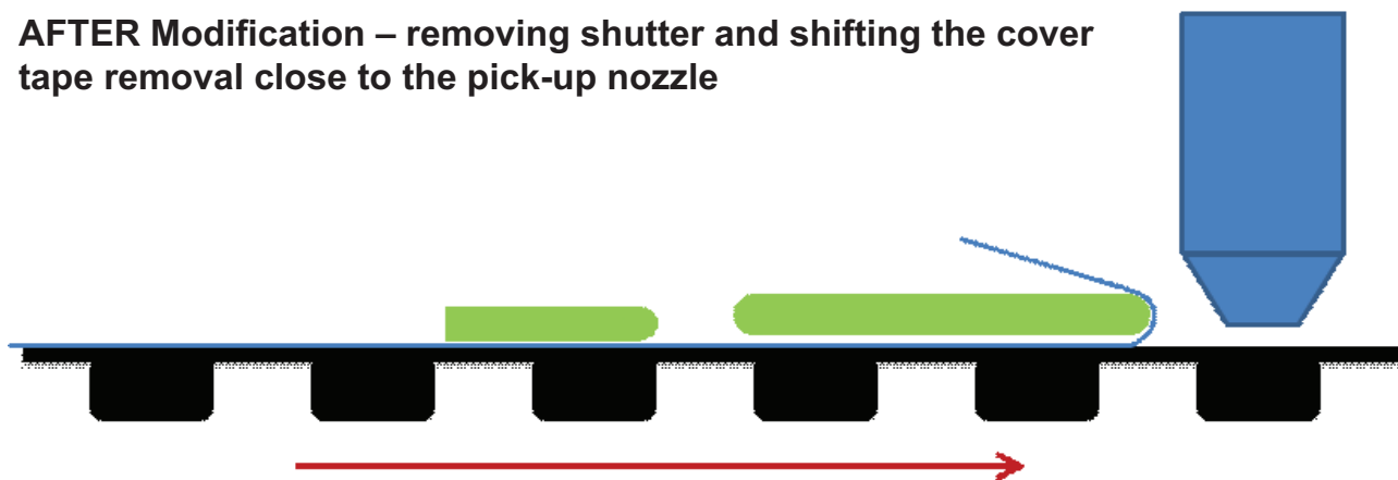
Figure 38. Minor modifications to the pick and place machine minimize the chance of damage to the dome of LUXEON Rebel.
