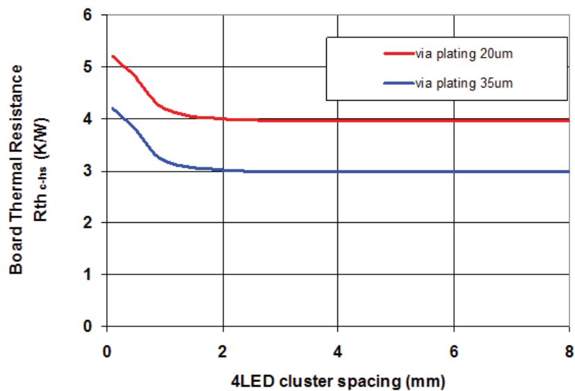
Figure 23. R_{\theta_{c-hs}} values of the PCB for different LED spacing and different via plating thicknesses.
