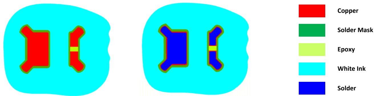
Figure 29. Recommended layout for LUXEON Rebel on MCPCB. Note that this layout is similar to the FR4 layout in Figure 8 but without all the vias.
