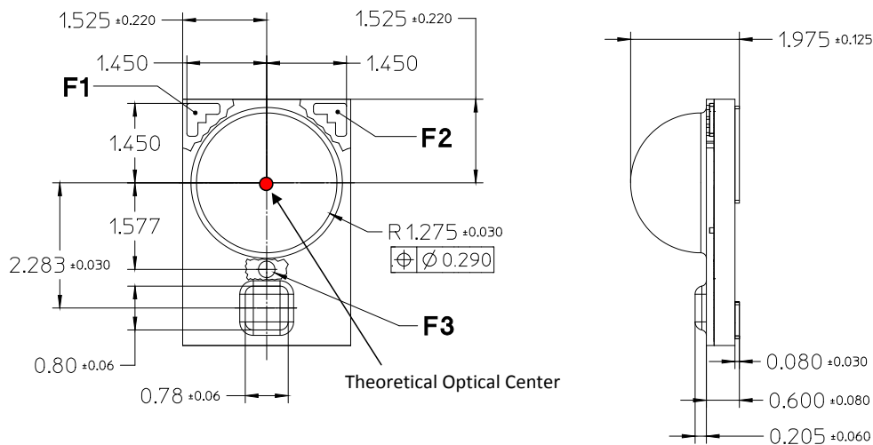
Figure 4. The fiducial marks on the front side of the LUXEON Rebel ES* package provide the most accurate method to find the theoretical optical center. Dimensions in mm.
