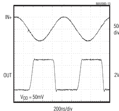
1MHz RESPONSE
