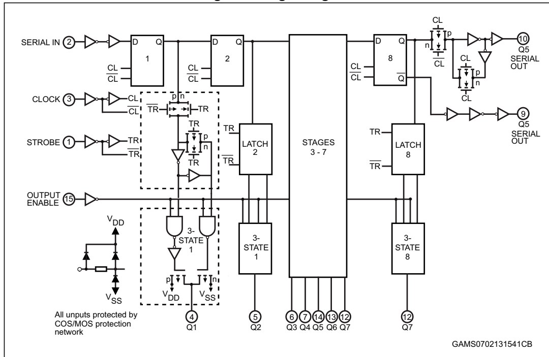
Figure 2. Logic diagram
