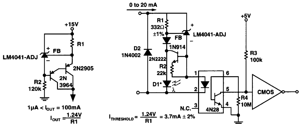
Figure 10. Current Source
