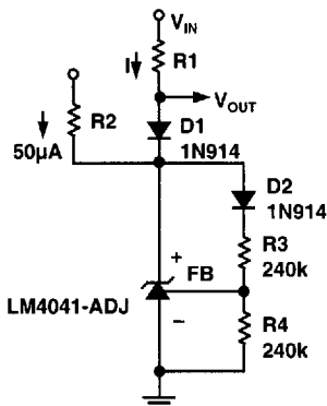
Figure 5. Fast Positive Clamp 2.4\text{V} + \Delta V_{D1}
