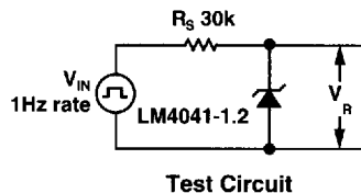
Test Circuit
