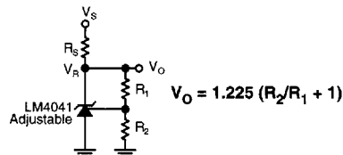
Figure 2. LM4041 Adjustable Shunt Regulator Application
