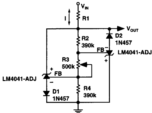
Figure 7. Bidirectional Adjustable Clamp \pm 18\text{V} to \pm 2.4\text{V}
