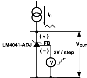
† Reverse Characteristics Test Circuit
