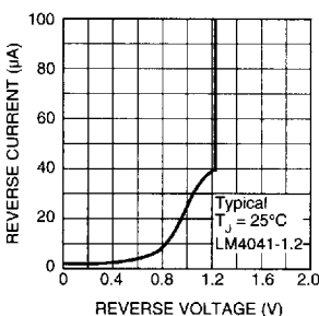
Reverse Characteristics and Minimum Operating Current
