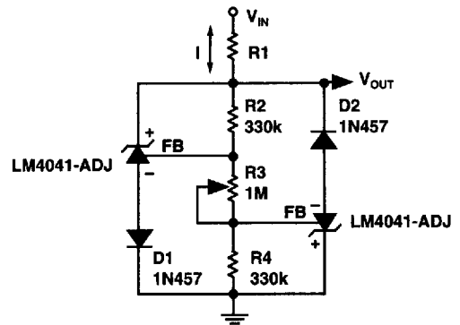
Figure 8. Bidirectional Adjustable Clamp \pm 2.4 to \pm 6\text{V}
