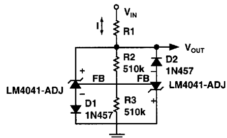
Figure 6. Bidirectional Clamp \pm 2.4\text{V}
