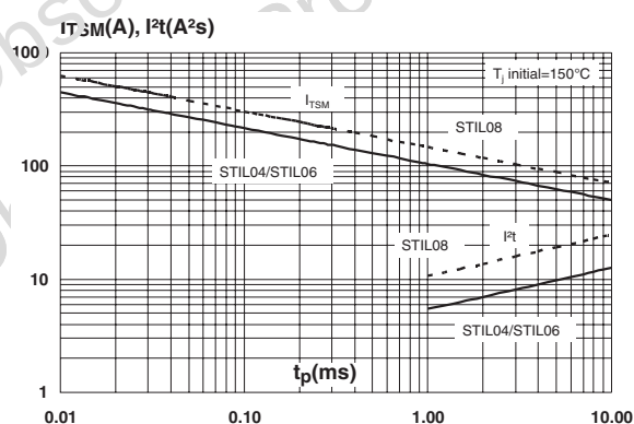
Figure 10: Non-repetitive surge peak on-state current (sinusoidal pulse) and corresponding value of \theta_{JA} (initial = 150°C)
