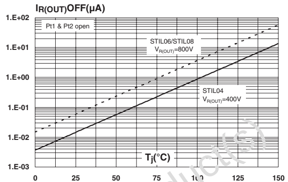
Figure 14: Reverse current versus junction temperature without driver current (typical values)
